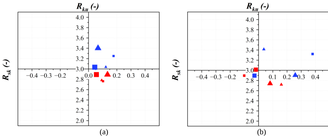
Figure 16. Skewness ( R_{sk} ) versus kurtosis ( R_{ku} ) for side measured surfaces under varied machining conditions (a) plunge milling, (b) face milling.
