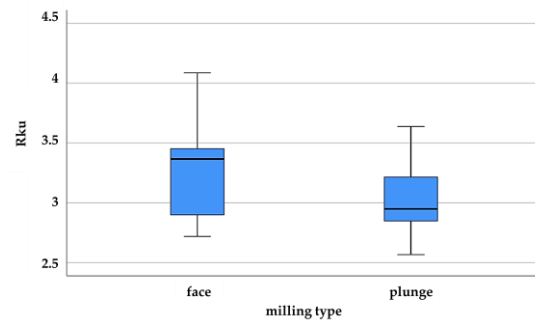
Figure 14. Boxplots of Surface Roughness R_{ku}
