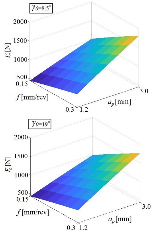
Figure 5. Surface plot (3D plot) of the main cutting force ( F_c ) for different rake angles ( \gamma_0 ) application. Conversely, an increase in feed rate also
