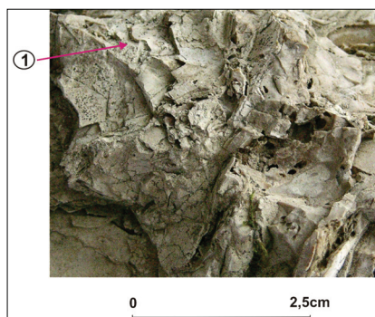
Photo 3b. Enlarged picture of porous spring deposits. – 1 = 0.5 mm thin sheets
