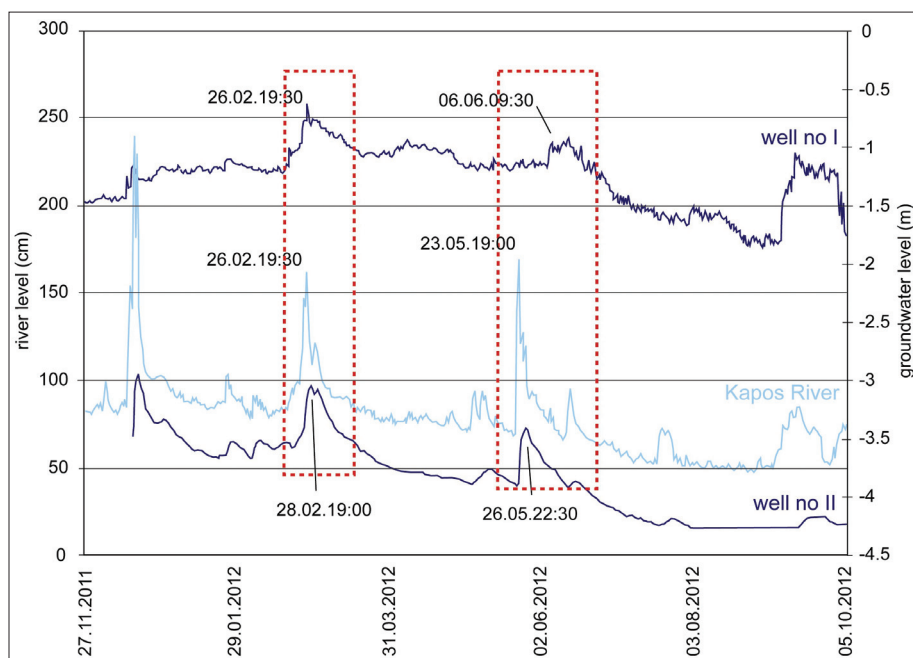
Fig. 5. River stages of the Kapos River at the Kurd gauge and groundwater levels recorded in observation wells I (Kurd) and II (Dúzs) between November 2011 and October 2012 (by DEZSŐ, J. 2012)
