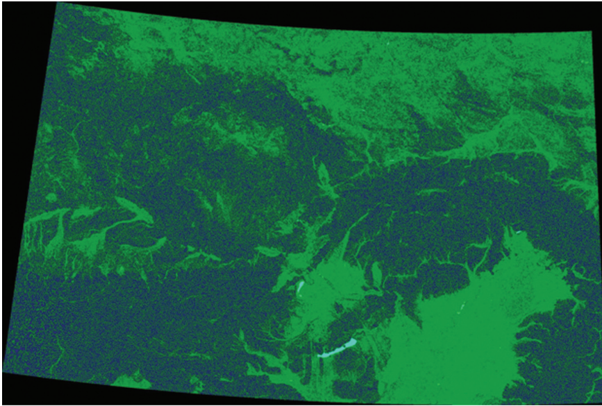
Fig. 5. Colluvial areas colored dark blue (curvature<0, slope%>2)
