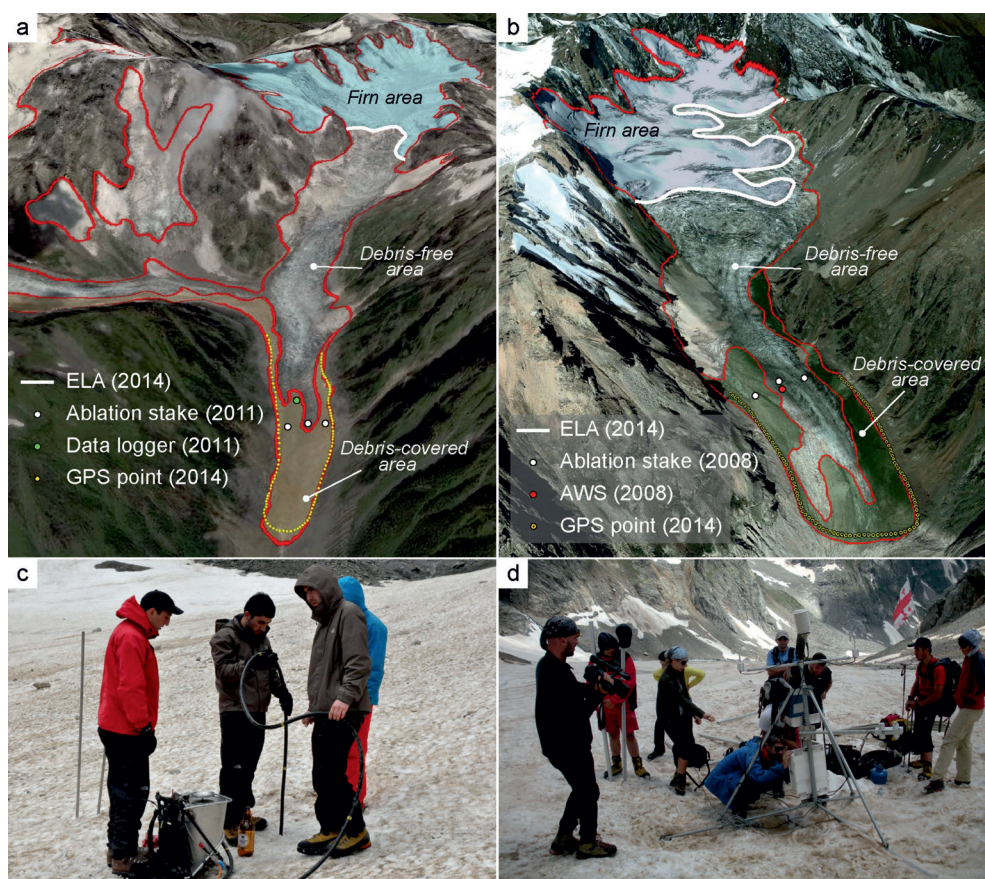
Fig. 3. Example of glacier mapping. – a = Chalaati Glacier – GeoEye (2012) image is used as the background; b = Zopkhito Glacier – Google Earth (19/09/11) image is used as the background; c = Ablation stake installation onto the Chalaati Glacier; d = Automatic Weather Station (AWS) installation onto the Zopkhito Glacier
