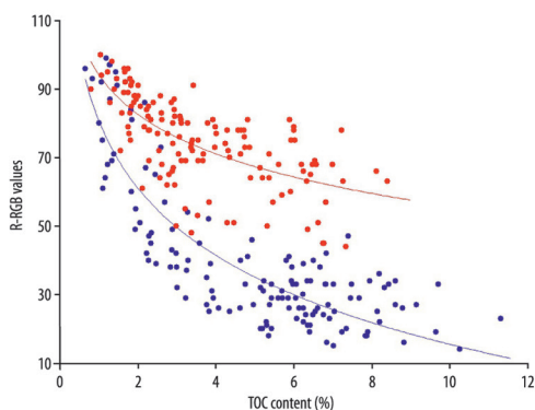
Fig. 3. The influence of TOC content on R-RGB values in soils samples of chernic (blue circles, n = 147 ), and mollic + umbric (red circles, n = 147 ) soil horizons
