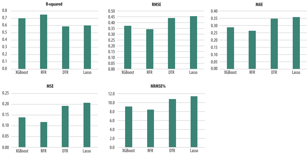
Fig. 6. Performance metrics of several ML models
