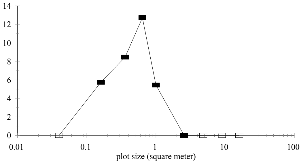
Figure 8. G(AB, AC, BC) -statistic as a function of scale. Filled squares mark field data significantly different from random, empty squares field data not different from random, filled triangles: upper and lower bound of 95% confidence interval.
