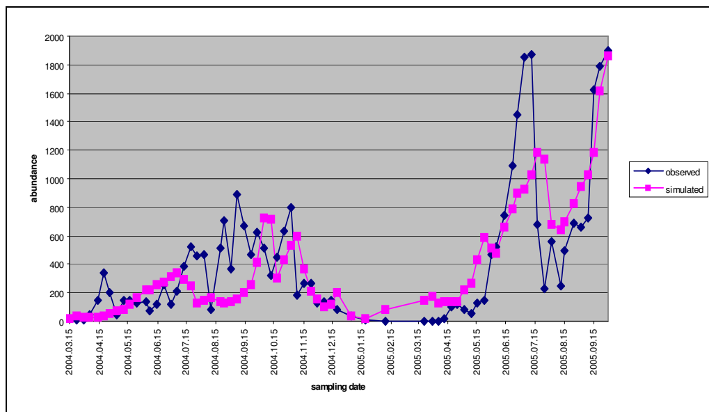
Figure 4. The observed and simulated individual numbers by cyclopoids during the survey.
