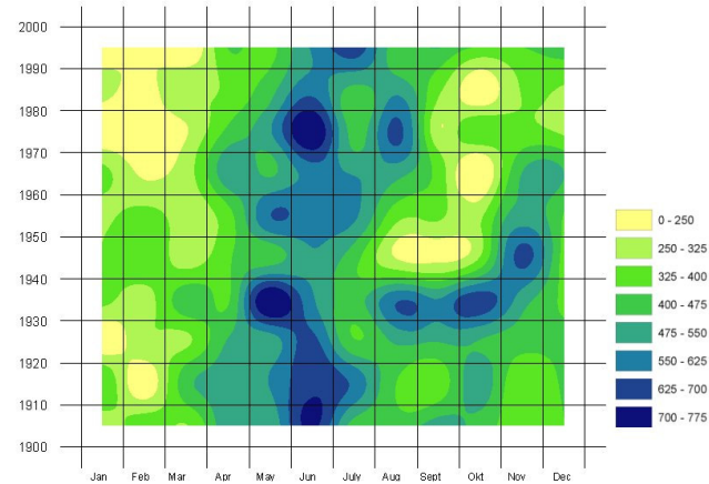
Figure 5. Monthly precipitation changes with interpolation methods
