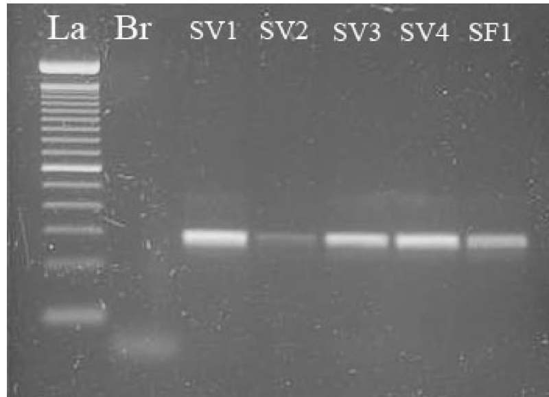
Figure 5. A 1,5% agarose gel including a 100 bp ladder (La), and the negative control (Br) Fragments of 300 bp correspond to the amplification product of the partial mcxA gene from samples from the São Francisco Verdadeiro (SV1, SV2, SV3 and SV4) and São Francisco Falso (SF1) tributaries, using the mcxA -Cd1R and mcxA -Cd1F primers
