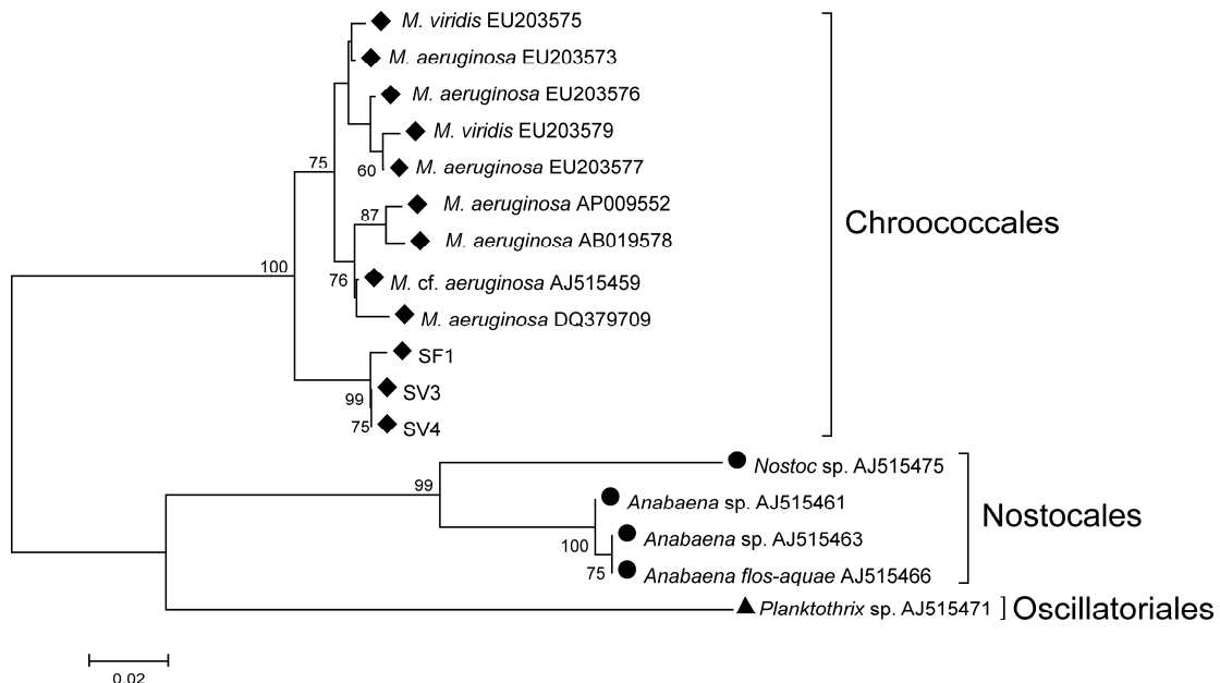
Figure 6. Neighbor-Joining tree built with the p distance, with 10,000 bootstrap, using sequences of the partial mcxA gene from samples of cyanobacteria blooms from the São Francisco Verdadeiro (SV3 and SV4) and São Francisco Falso (SF1) tributaries and sequences available in GenBank
