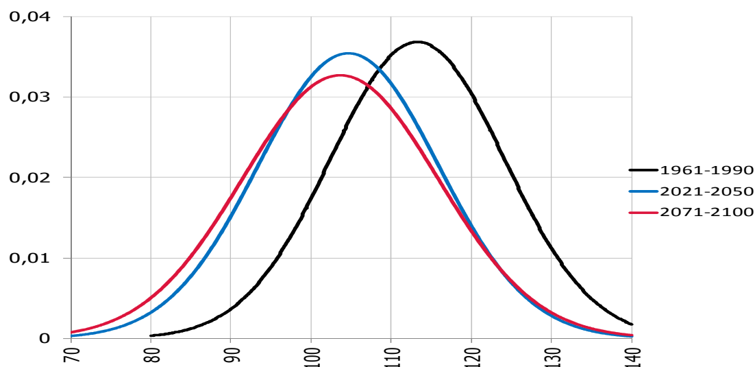
Figure 5. Fitted normal distribution curves for the budburst dates predicted by the regional climate model RegCM 3.1 for time intervals 1961-1990, 2021-2050 and 2071-2100
