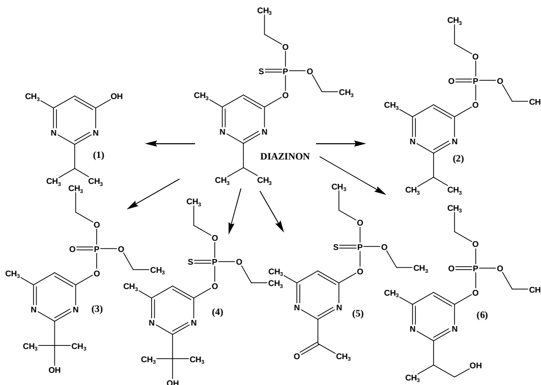
Figure 2. Scheme of the proposed photodegradation pathway for diazinon: 2-isopropyl-6-methyl-pyrimidin-4-ol, (IMP) (1), dizoxon (2), hydroxydizoxon (3), hydroxydiazinon (4) diazinon methyl ketone (5), 2-hydroxydiazoxon (6)
