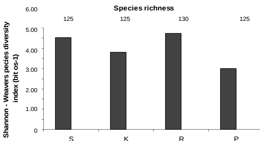
Figure 6. Species diversity Shannon-Weaver's coefficients for periphyton assemblages (S – periphyton in separator pipes, K – epilithon, R – epiphyton) and phytoplankton (P – pelagial) in Lake Jeziorak Mały in the years 1997-2003 and 2005
