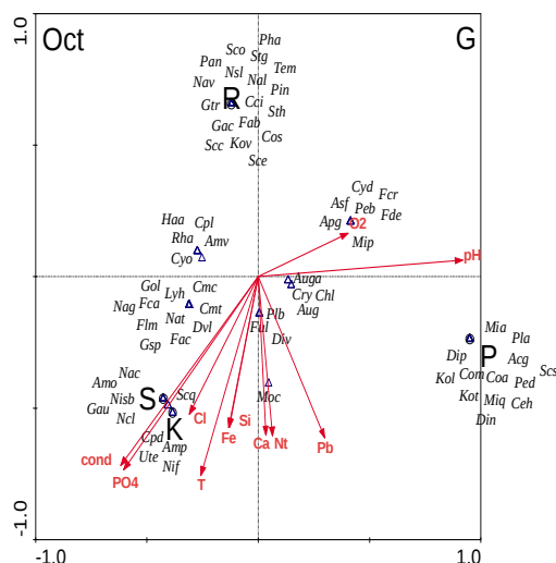
Figure 7. Tri-plots ordination diagram of Canonical Correspondence Analysis (CCA) showing the relationships between periphyton assemblages (S – periphyton in separator pipes, K – epilithon, R – epiphyton) and phytoplankton (P – pelagial) and physicochemical water parameters in the season from April to October (A-G) in Lake Jeziorak Mały (Aca – Actinastrum aciculare , Ach – Actinastrum hantzschii , Acg – Actinastrum gracilimum , Aml – Amphora libyca , Amo – Amphora ovalis , Amp – Amphora pediculus , Amv – Amphora veneta , Anc – Anabaena crassa , Ans – Anabaena smithii , Apf – Aphanizomenon flos-aquae , Apg – Aphanizomenon gracile , Asf – Asterinella formosa , Aug – Aulacoseira granulata , Auga – Aulacoseira granulata var. angustissima , Caa – Caloneis amphisbaena , Chl – Chlamydomonas spp., Ceh – Ceratium hirundinella , Clp – Closterium pronum , Cpd – Cocconeis pediculus , Cpl – Cocconeis placentula , Coa – Coleastrum astroideum , Com – Coleastrum microporum , Cos – Cosmarium sp., Cry – Cryptomonas sp., Cyd – Cyclostephanos dubius , Cyc – Cyclotella comta , Cyo – Cyclotella ocellata , Cci – Cymbella cistula , Cmc – Cymbella compacta , Cmm – Cymbella microcephalla , Cms – Cymbella silesiaca , Cmt – Cymbella tumida , Dih – Diatoma hyemalis , Div – Diatoma vulgaris , Dvl – Diatoma vulgaris var. linearis , Dip – Dictyosphaerium pulchellum , Din – Dinobryon sp., Dio – Diploneis ovalis , Epa – Epithema adnata , Ept – Epithema turgida , Eud – Eudorina sp., Eua – Euglena acus , Euv – Euglena viridis , Fac – Fragilaria acus , Fab – Fragilaria biceps , Fca – Fragilaria capucina , Fcr – Fragilaria crotonensis , Fde – Fragilaria delicatissima , Flm – Fragilaria leptostauron var. martyi , Ful – Fragilaria ulna , Gor – Golenkinia radiata , Glc – Golenkiniopsis sp., Gac – Gomphonema acuminatum , Gau – Gomphonema augur , Glu – Gomphonema lungilatifforme , Gol – Gomphonema olivaceum , Gpa – Gomphonema parvulum , Gtr – Gomphonema truncatum , Gsp – Gomphonema spp., Gon – Gomphosphaeria naegeliana , Gyf – Gymnodinium fuscum , Haa – Hantzschia amphioxys , Kls – Klebsormidium subtile , Kob – Koliella bernina , Koe – Koliella elongata , Kol – Koliella longiseta , Kon – Koliella nivalis , Kot – Koliella tenuis , Kov – Koliella variabilis , Kmv – Komvophoron schmidlei , Lir – Limnithrix redekei , Lyh – Lyngbya hieronymussii , Mal – Mallomonas sp., Mva – Melosira varians , Meg – Merismopedia glauca , Mip – Micratinium pusillum , Miq – Micratinium quadrisetum , Mia – Microcystis aeruginosa , Mch – Microcystis ichtyoblabe , Mis – Microcystis smithii , Moc – Monoraphidium concertum , Monoraphidium griffithii, Moi – Monoraphidium irregulare , Nac – Navicula capitata , Ncl – Navicula clementis , Nag – Navicula gregaria , Nal – Navicula lanceolata , Nre – Navicula reinhardtii , Nrh – Navicula rhynchotella , Nsl – Navicula slesvicensis , Nat – Navicula tripunctata , Nav – Navicula viridula , Nif – Nitzschia frustulum , Nil – Nitzschia linearis , Nis – Nitzschia sigmaidea , Nisb – Nitzschia sublinearis , Niu – Nitzschia uwellerstorffii , Osl – Oscillatoria limosa , Pan – Pandorina sp., Peb – Pediastrum boryanum , Ped – Pediastrum duplex , Pei – Peridinium inconspicuum , Pes – Peridinium sp., Pha – Phacus sp., Pho –
