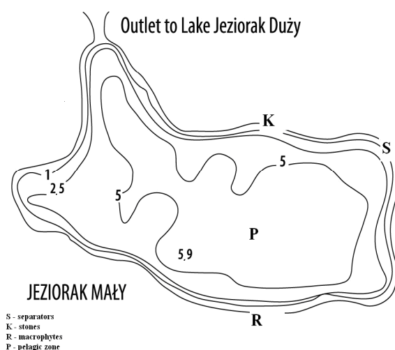
Figure 1. Morphometric map of Lake Jeziorak Mały
