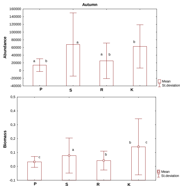
Figure 4. Differentiation of abundance (A) and biomass (B) of periphyton assemblages (S – periphyton in separator pipes, K – epilithon, R – epiphyton) and phytoplankton (P – pelagial) in autumn (Tukey test, ANOVA) in Lake Jeziorak Mały in the years 1997-2003 and 2005
