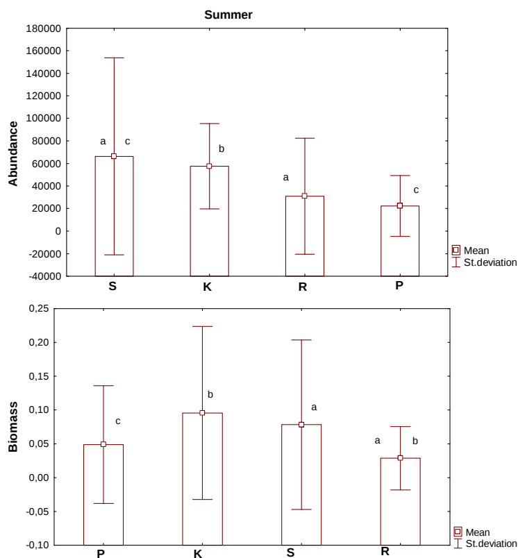
Figure 3. Differentiation of abundance (A) and biomass (B) of periphyton assemblages (S – periphyton in separator pipes, K – epilithon, R – epiphyton) and phytoplankton (P – pelagial) in summer (Tukey test, ANOVA) in Lake Jeziorak Mały in the years 1997-2003 and 2005
