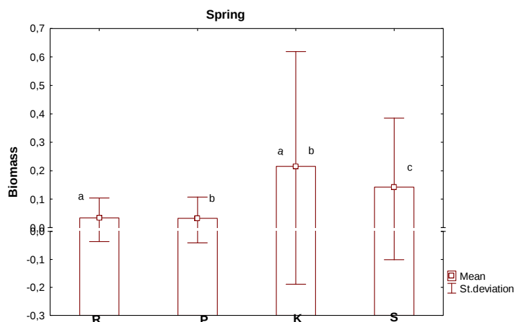
Figure 2. Differentiation of biomass of periphyton assemblages (S – periphyton in separator pipes, K – epilithon, R – epiphyton) and phytoplankton (P – pelagial) in spring (Tukey test, ANOVA) in Lake Jeziorak Mały in the years 1997-2003 and 2005
