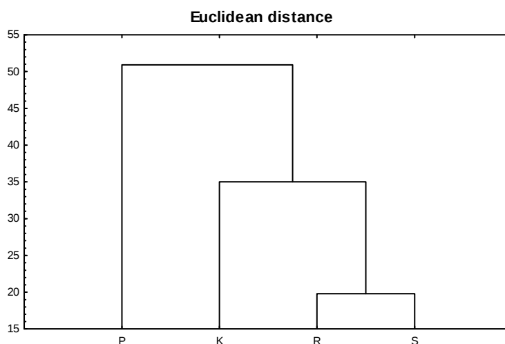
Figure 5. Dendrogram of Euclidean distances between periphyton assemblages (S – periphyton in separator pipes, K – epilithon, R – epiphyton) and phytoplankton (P – pelagial) in Lake Jeziorak Mały in the years 1997-2003 and 2005
