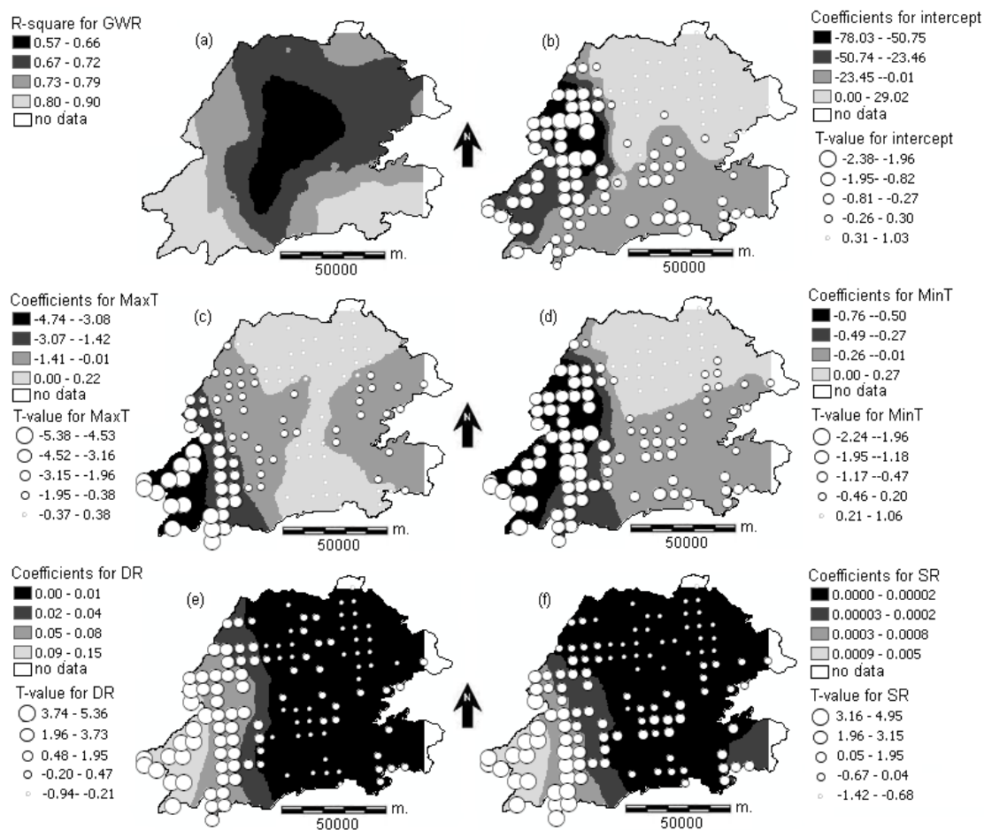
Figure 4. a. Locally variable R-square for GWR; estimated coefficients and t-values for significant predictors of GWR model including b. Intercept of the model; c. Maximum temperature of July (MaxT); d. Minimum temperature of January (MinT); e. Diurnal Range (DR); f. Solar Radiation (SR)
