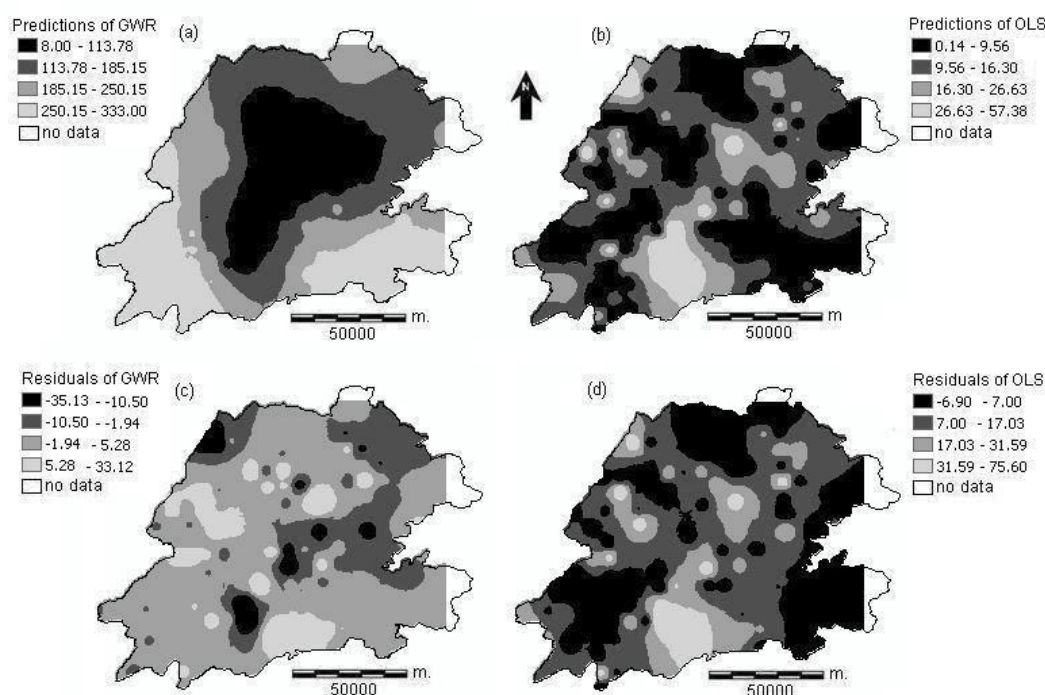
Figure 2. a. Distribution of butterfly species richness predicted by GWR model; b Distribution of butterfly species richness predicted by OLS regression model; c Residuals from GWR model; d Residuals from OLS regression model
