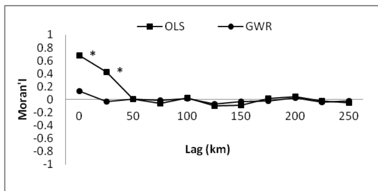
Figure 5. Spatial autocorrelation of model residuals for the GWR and OLS regression models, (* P values; 0.01 < P < 0.05 )
