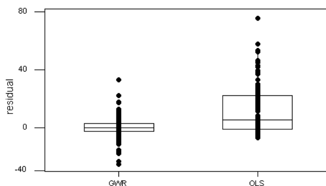
Figure 3. Box-plot for residuals of local GWR and global OLS models
