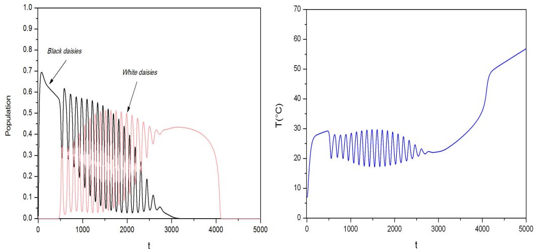
Figure 9. Daisyworld response with linear increase solar luminosity ( 0.75 \leq \bar{L} \leq 1.7 ; L_0 = 0 ), greenhouse gases variable ( 0.0 \leq G \leq 0.8 ) and c = 300 \text{ J/m}^2\text{K s}
