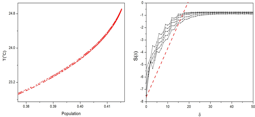
Figure 35. Chaotic response for \bar{L} = 1.05 (same situation presented in Figure 36). Poincaré section (left) and respective maximum Lyapunov exponent (right)
