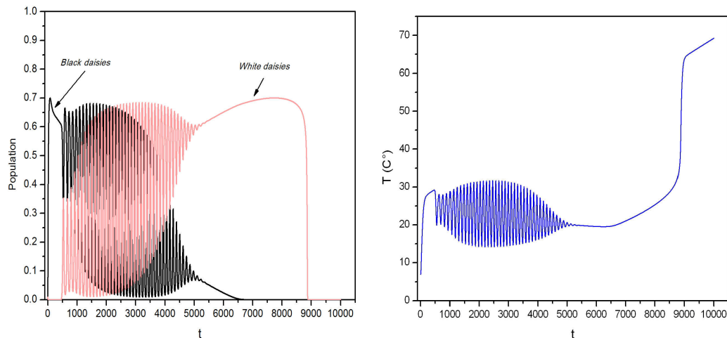
Figure 5. Daisyworld response with linear increase solar luminosity ( 0.75 \leq \bar{L} \leq 1.7 ; L_0 = 0 ) and c = 300 \text{ J/m}^2\text{K s} . Daisy population (left) and the temperature (right)
