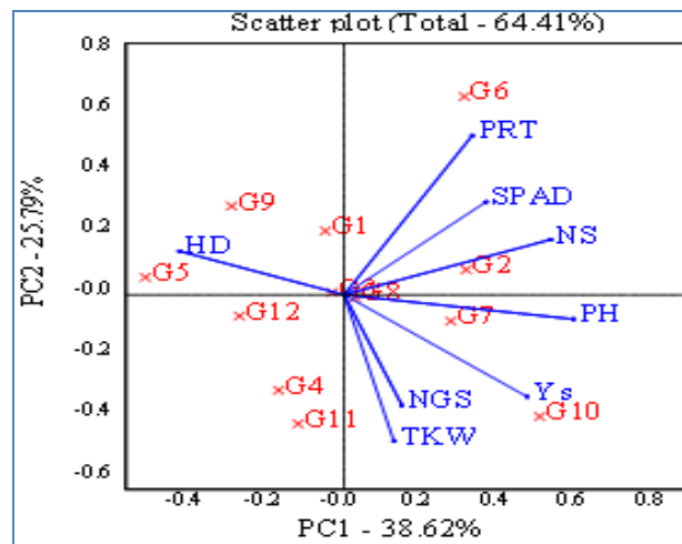
Figure 2. Biplot based on first two principal component axes (PC1 and 2) for traits of genotypes in rain-fed conditions.
