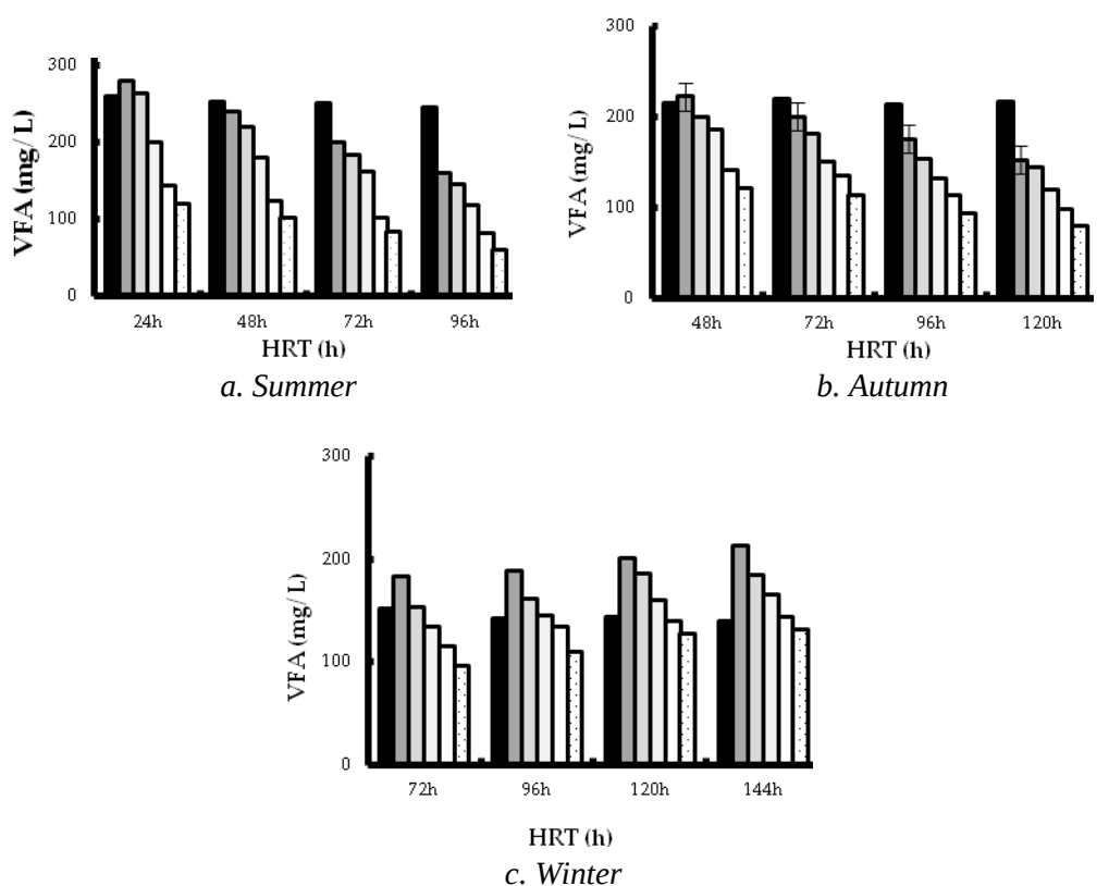
Figure 6. VFA removal efficiency of ABR under different HRTs Inflow ■ Compartment I ■ Compartment II ■ Compartment III ■ Compartment IV ■ Compartment V ■
