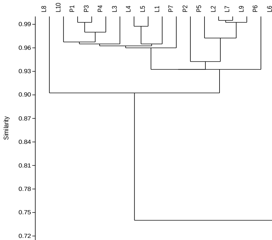
Figure 2. Raup Crick cluster diagram showing site similarities / dissimilarities among pelagic (P) and littoral (L) sites sampled in the Manjirenji Dam.
