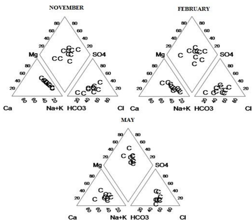
Figure 2. Piper trilinear diagram for groundwater samples
