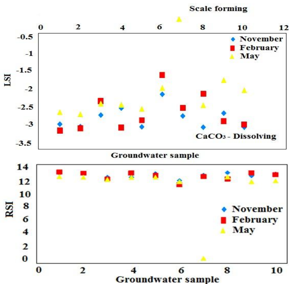
Figure 6. LSI and RSI of groundwater samples
