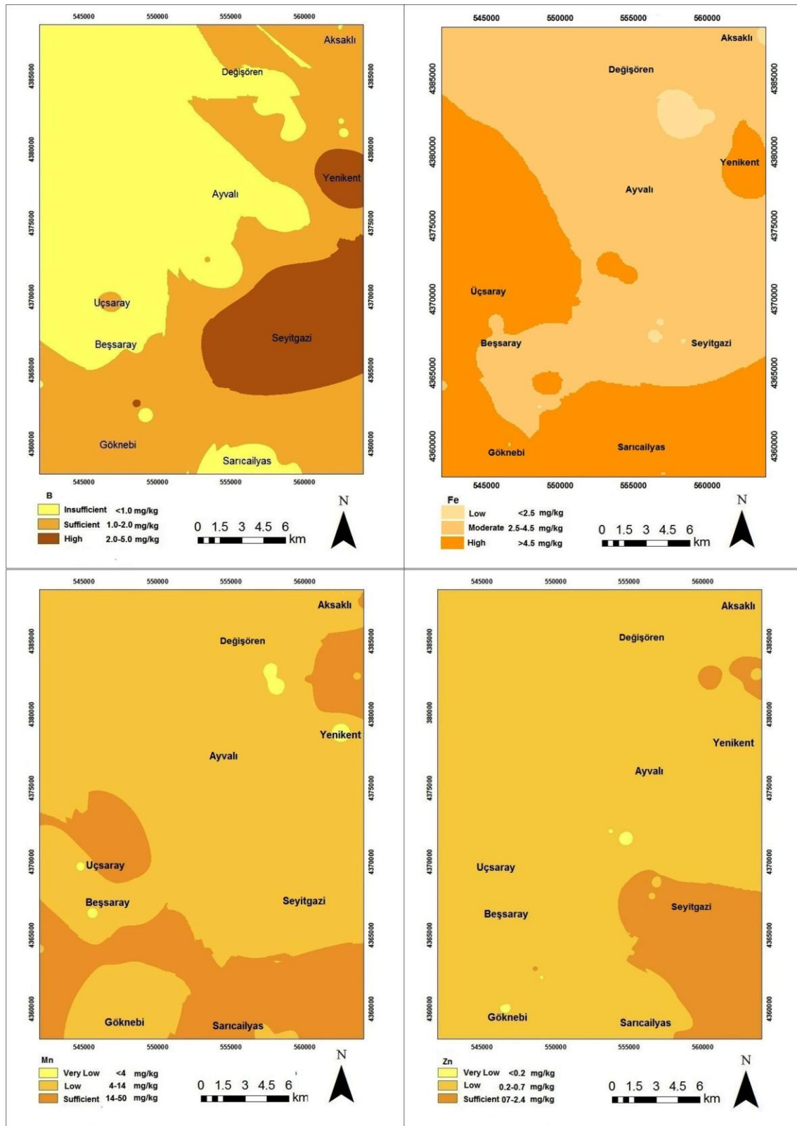
Figure 2. Spatial distribution maps of available B, Fe, Mn and Zn concentrations of samples by distance from Kirka Boron Mine
