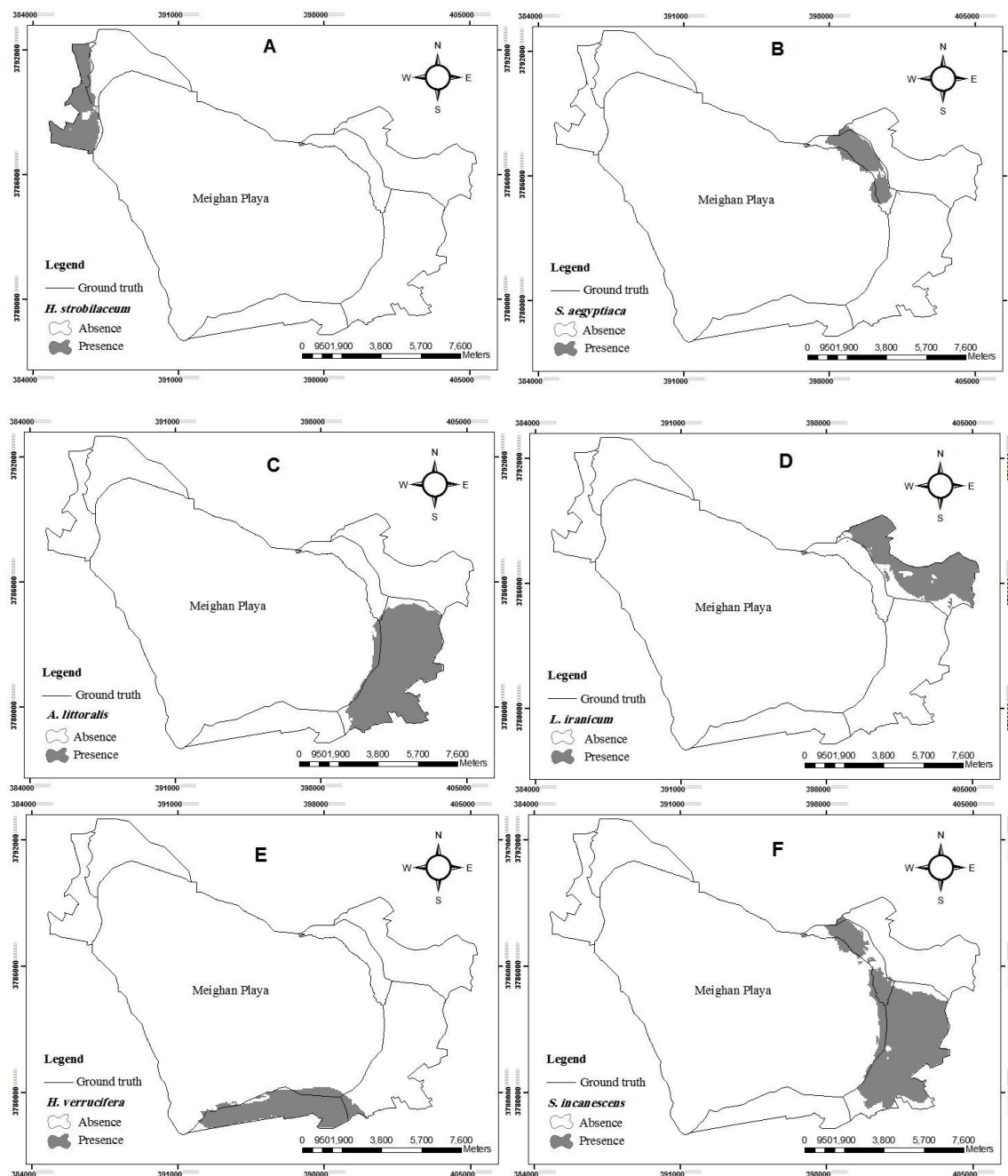
Figure 2. Actual and predicted species distribution maps for A: Halocnemum strobilaceum , B: Suaeda aegyptiaca , C: Aeluropus littoralis , D: Limonium iranicum , E: Halimione verrucifera and F: Salsola incanescens (predictive maps is shown darker)
