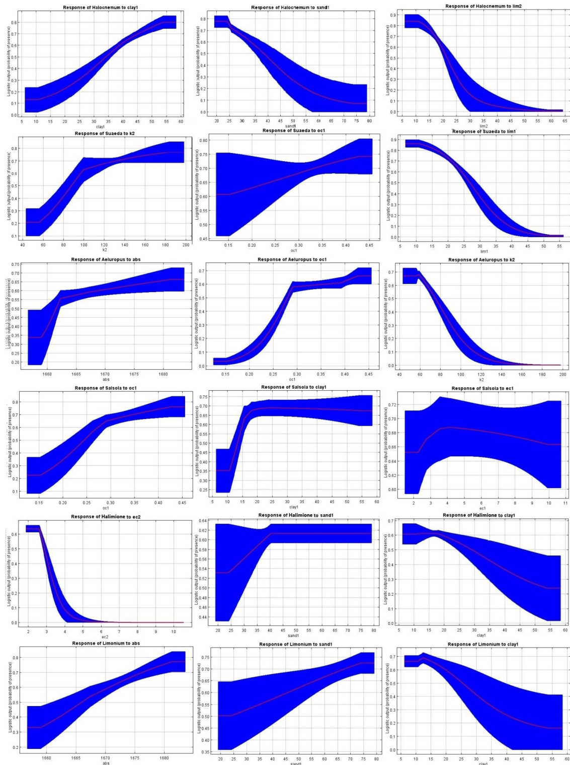
Figure 3. Most important response curves of species to environmental variables
