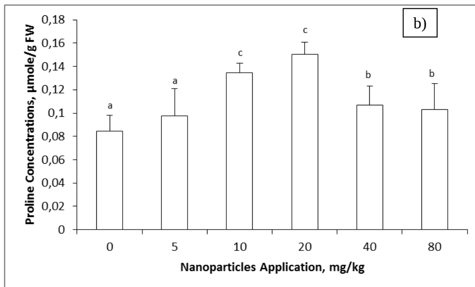
Figure 4. The proline concentrations of wheat plants, a) TiO 2 and b) ZnO nanoparticles (The significance between the groups indicate with different letters)
