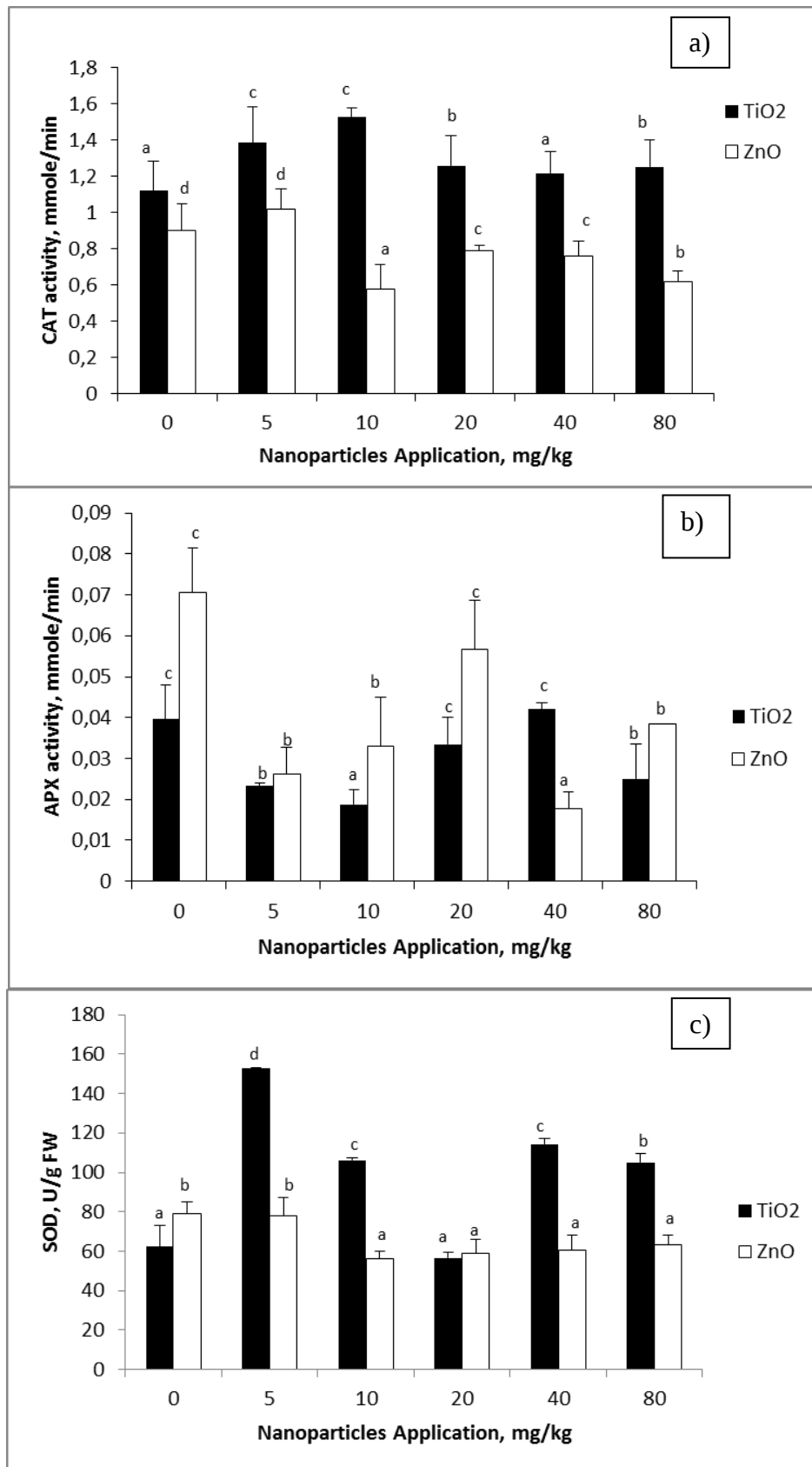
Figure 3. a) Catalase (CAT), b) Ascorbate peroxidase (APX) and c) Superoxide dismutase (SOD) activities in wheat (The significance between the groups indicate with different letters)
