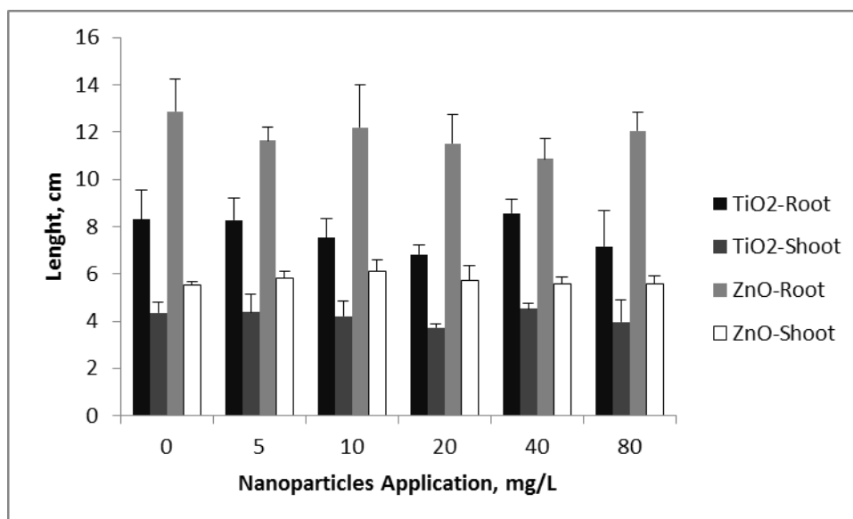
Figure 1. Effect of different TiO 2 and ZnO nanoparticles concentrations on root and shoot elongation of wheat (The significance between the groups indicate with different letters)
