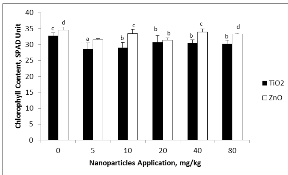
Figure 2. Effect of different TiO 2 and ZnO nanoparticles concentrations on chlorophyll content (in SPAD units) of wheat (The significance between the groups indicate with different letters)
