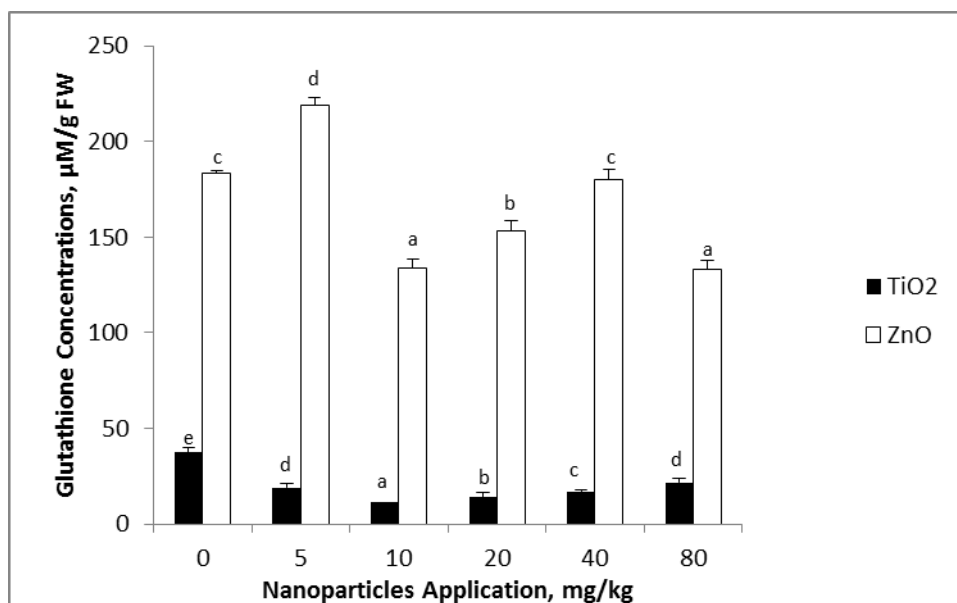
Figure 5. Glutathione concentrations of wheat plants (The significance between the groups indicate with different letters)
