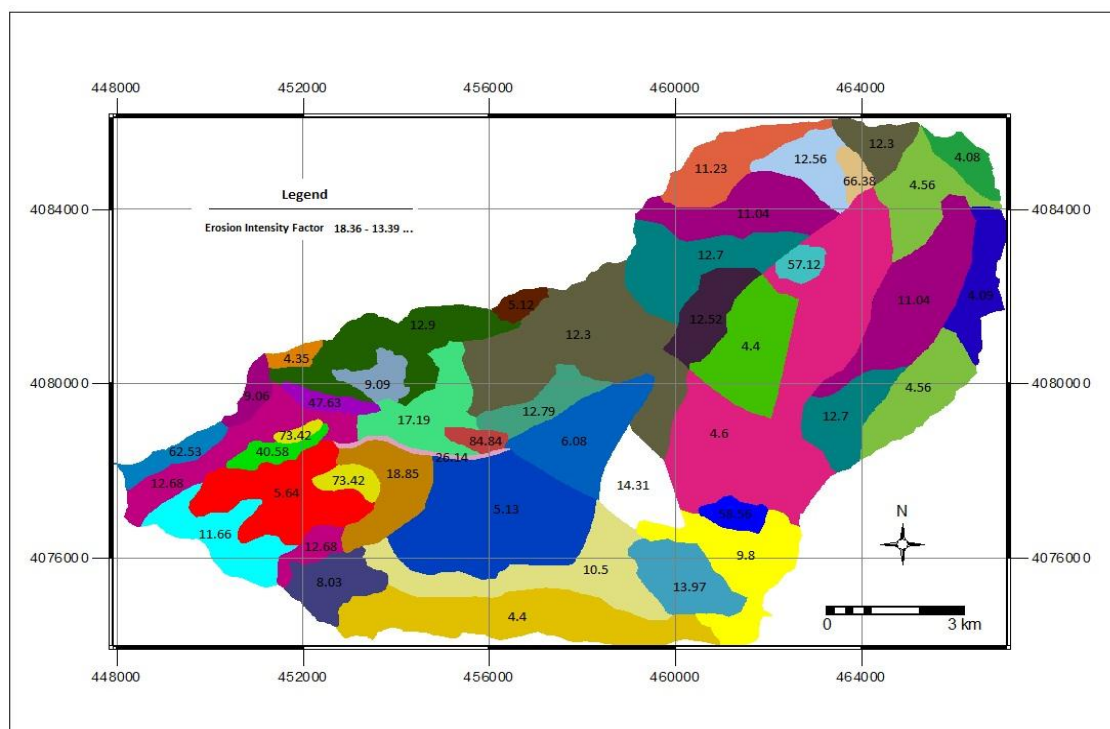
Figure 3. Erosion intensity map at the base time after project implementation (2014).
