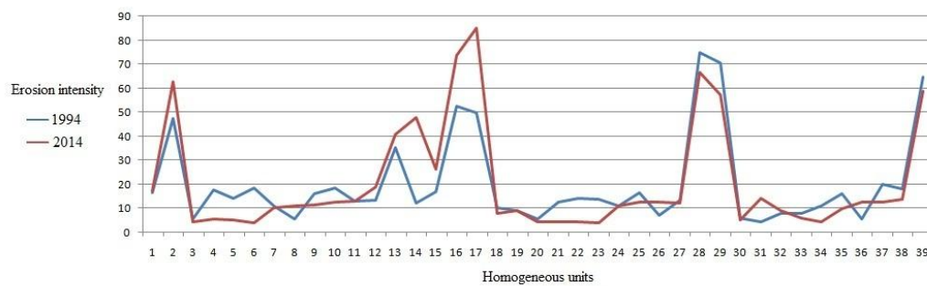
Figure 4. Erosion intensity change
