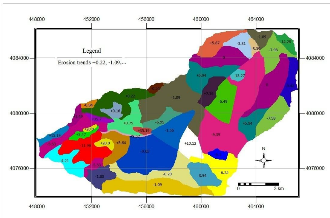
Figure 5. Map of erosion trends.
