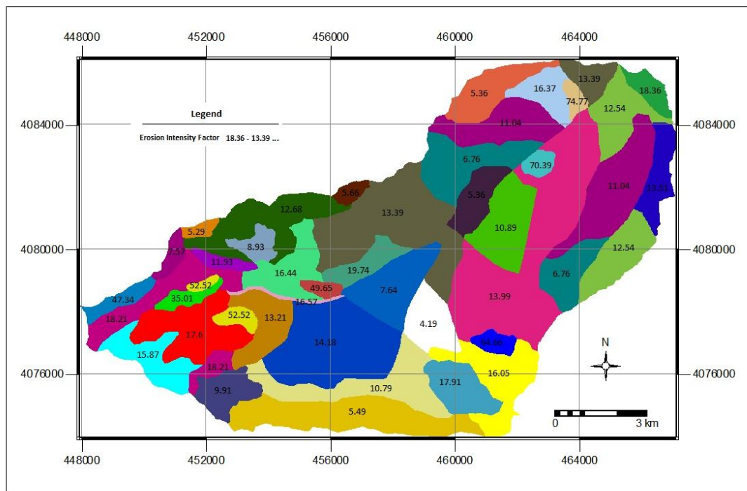
Figure 2. Erosion intensity map at the base time before project implementation (1994).
