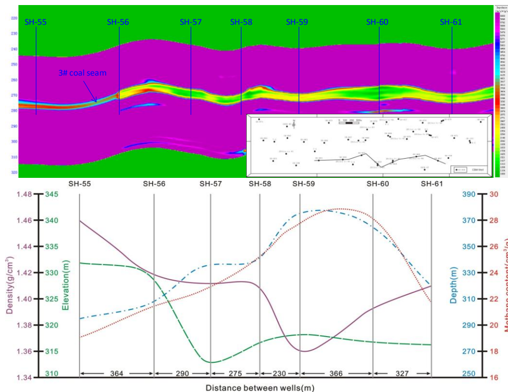
Figure 11. The section correlogram between SH-55 and SH-61
