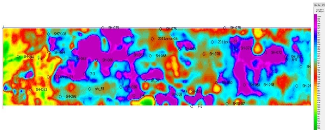
Figure 8. The impedance inversion map of roof stratum of 3# coal
