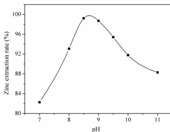
Figure 5. Effect of pH on the extraction efficiency of Zn(II) ions. CPE conditions: Zn(II), (100 ng/mL); saturated NaCl, 1.2 mL; SDS 0.1% (w/w); Triton X-100, 0.4% (v/v) and PAN, 0.14 mL ( 4 \times 10^{-3} mol/L)
