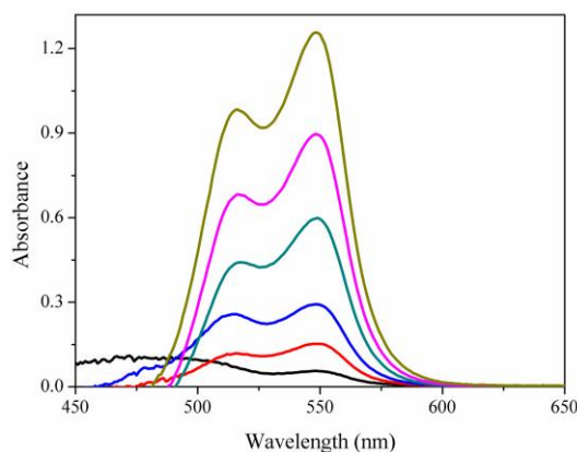
Figure 2. Absorption spectra of different concentrations of Zn(II)-PAN complex after CPE
