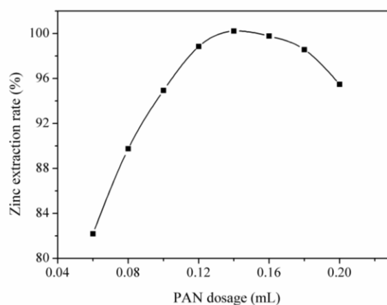
Figure 6. Effect of PAN dosage on the extraction efficiency of Zn ( II) ions. CPE conditions: Zn( II), (100 ng/mL); saturated NaCl, 1.2 mL; SDS 0.1% (w/w); Triton X-100, 0.4% (v/v) and pH=8.5
