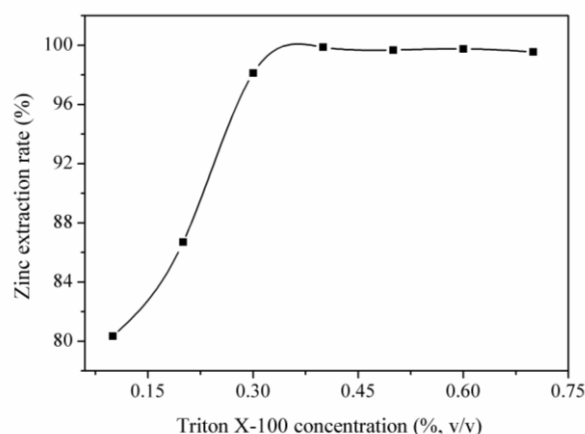
Figure 7. Effect of Triton X-100 concentration on the extraction efficiency of Zn( II) ions. CPE conditions: Zn( II), (100 ng/mL); saturated NaCl, 1.2 mL; SDS 0.1% (w/w); PAN 0.14 mL ( 4 \times 10^{-3} mol/L) and pH=8.5
