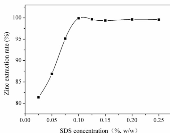
Figure 4. Effect of SDS concentration on the extraction efficiency of Zn (II) ions. CPE conditions: Zn(II), (100 ng/mL); saturated NaCl, 1.2 mL; Triton X-100, 0.4% (v/v); PAN, 0.14 mL ( 4 \times 10^{-3} mol/L) and pH=8.5
