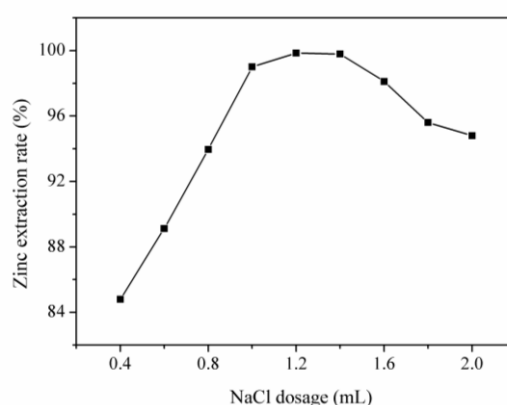
Figure 3. Effect of NaCl dosage on the extraction efficiency of Zn (II) ions. CPE conditions: Zn (II) (100 ng/mL); SDS 0.1% (w/w); Triton X-100, 0.4% (v/v); PAN, 0.14 mL ( 4 \times 10^{-3} mol/L) and pH=8.5
