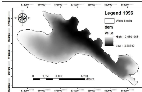
Figure 9. The DEM layer of water level in 1996
