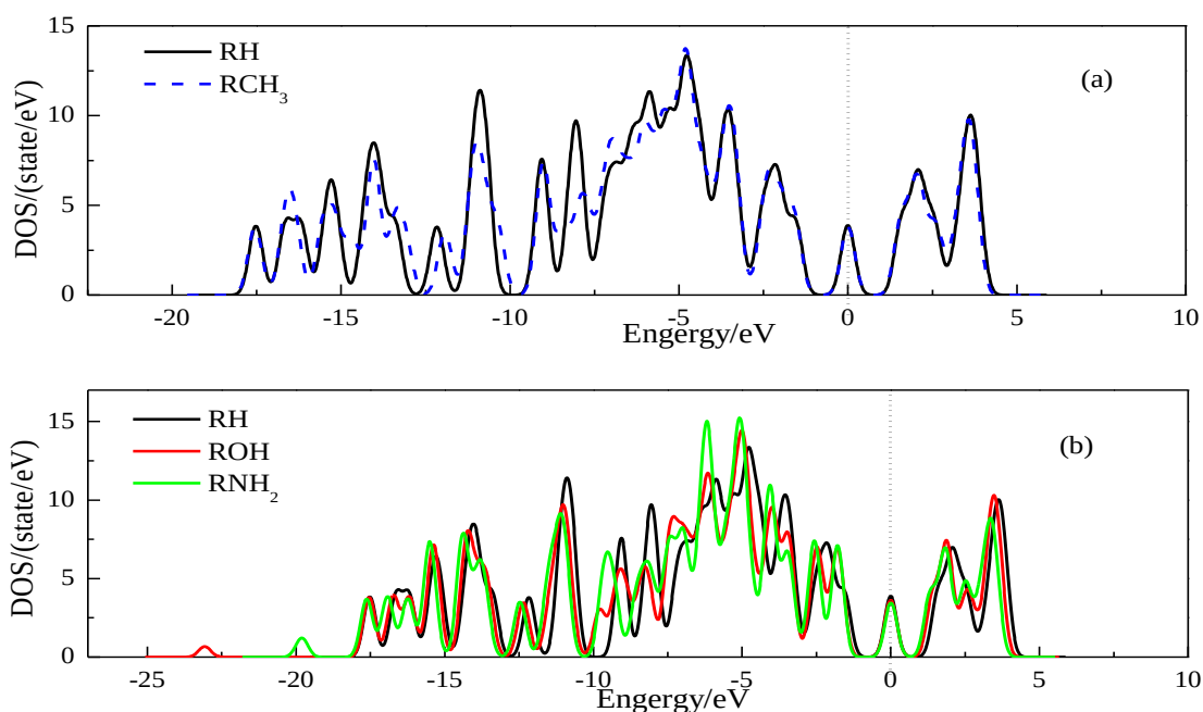
Figure 7. Density of states of the aromatic structure after methane adsorbing on B site of different kerogen fragments.
