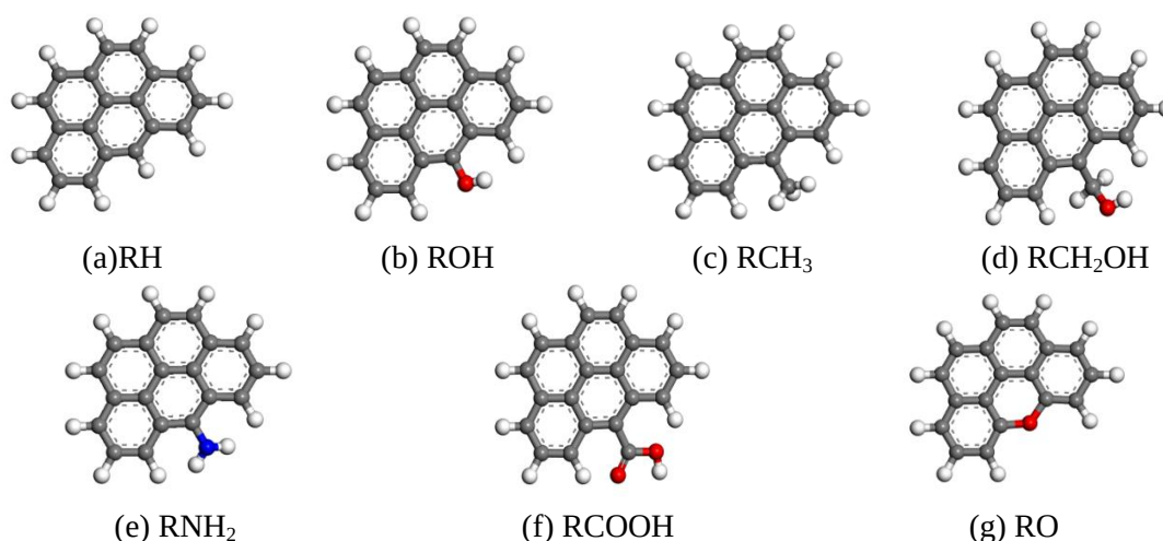
Figure 1. Kerogen fragments after optimization (Atoms representation: gray is for carbon atoms, white for hydrogen, red for oxygen, and blue for nitrogen).
