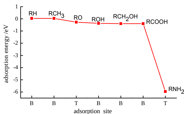
Figure 4. Adsorption energy of the most stable adsorption site of kerogen fragments.
