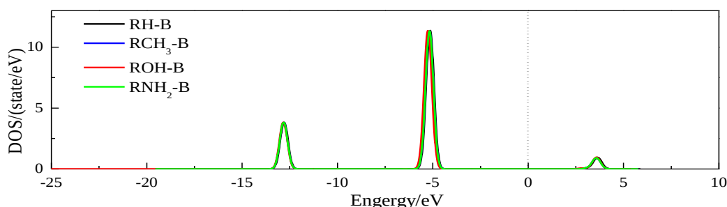
Figure 6. Density of states of methane after it adsorbing on B site of different kerogen fragments.
