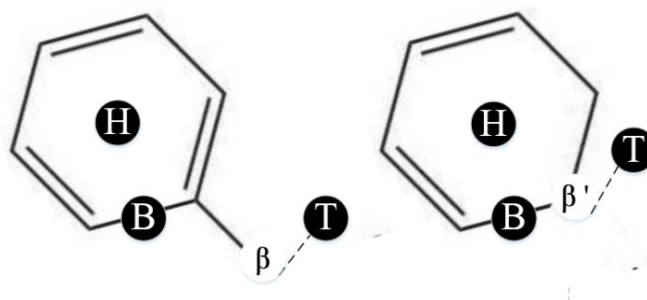
Figure 2. High-symmetry adsorption sites on the surface of Kerogen fragments ( \beta represents H, OH, CH 2 OH, COOH, CH 3 , NH 2 ; \beta' represents O).
