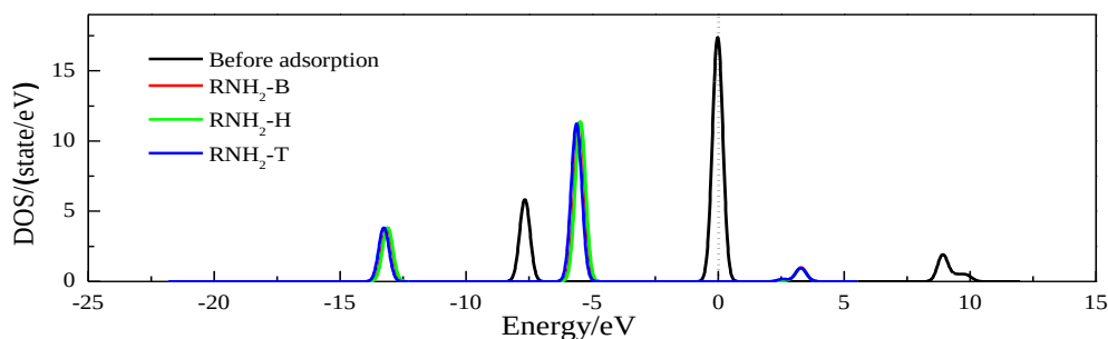
Figure 5. Density of states of methane before and after it adsorbing on the surface of kerogen fragment RNH 2 .
