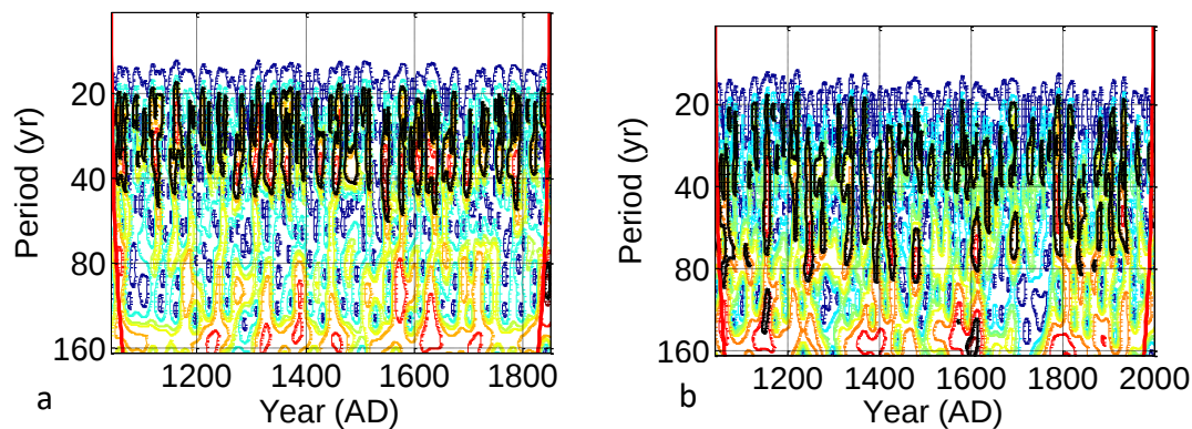
Figure 5. (a and b) Wavelet Transform module square time frequency distribution of depth of precipitation for CCSM4 model and ECHAM5 model. It was plotted by time series against periods, in which the 95% confidence contour was in black part and the red full line meant cone of influence. Any part below the red line is not reliable
