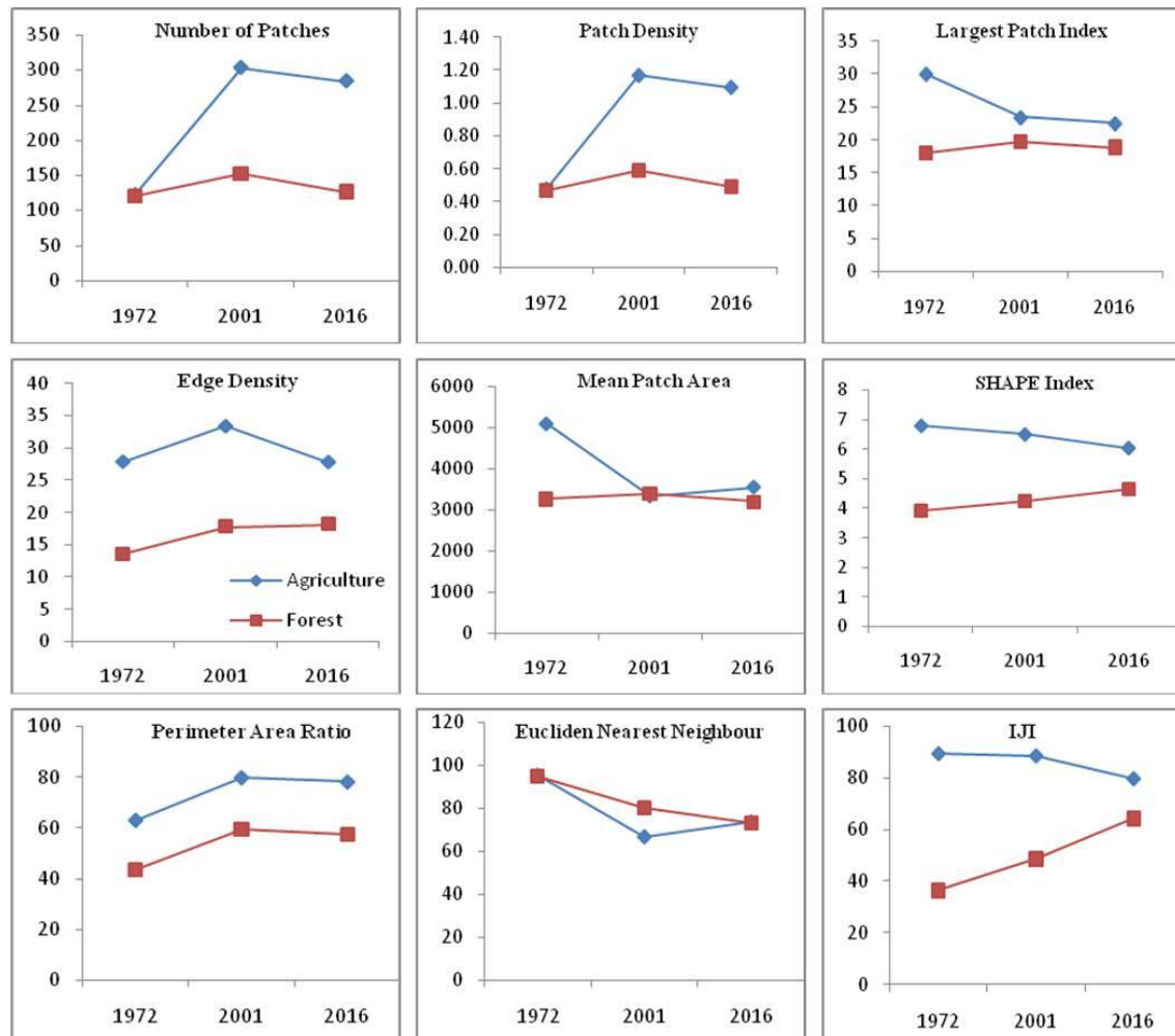
Figure 3. Temporal changes in the fragmentation metrics of forests and agriculture in the study area
