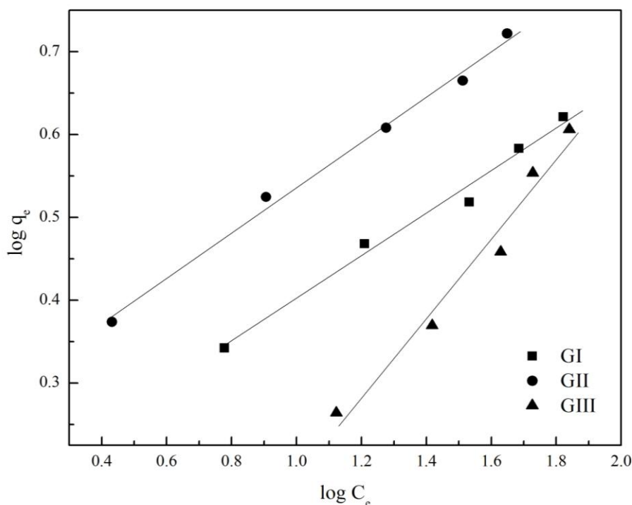
Figure 9. Freundlich adsorption isotherms for the adsorbents GI, GII and GIII
