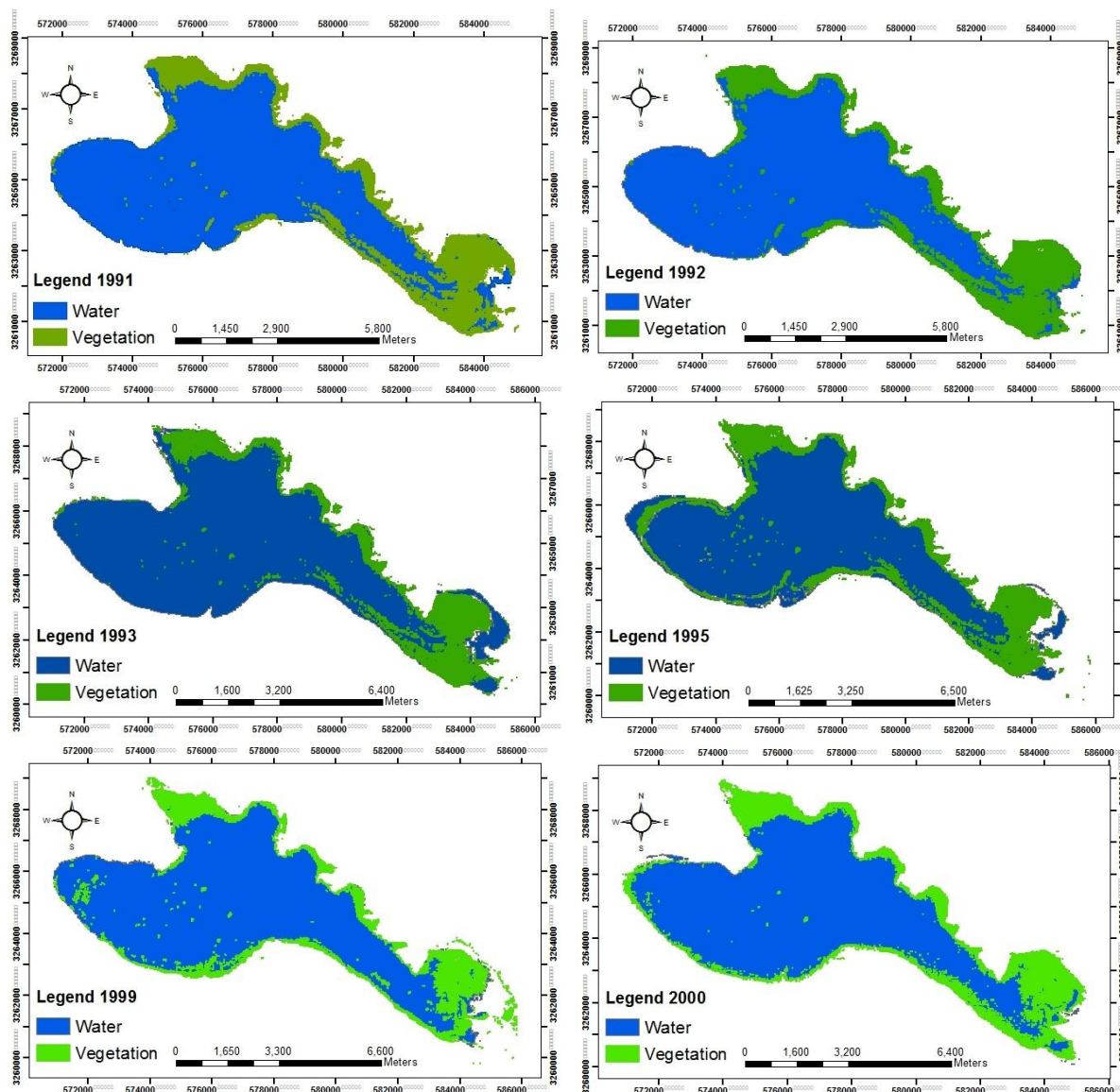
Figure 2. Classes of water and vegetation of Parishan wetland during the different years
