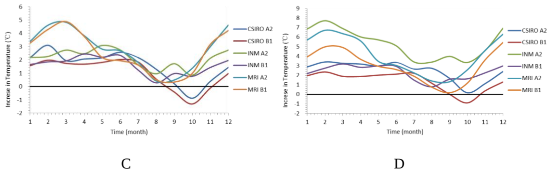
Figure 9. Changes of simulated monthly maximum (A and B) and minimum (C and D) temperature under scenarios A2 and B1 during the period of 2046-2065 and 2081-2100 respectively
