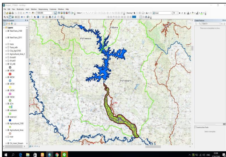
Figure 10. The flood area from the HEC-RAS model superimposed on a topographic map 1:50,000
