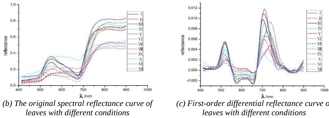
Figure 3. Comparison of spectral reflectance of leaves in different conditions. Curves I-XII. in Figure (b, c) are the original and first-order differential spectral curves corresponding to the leaves I-XII. in Figure (a).
