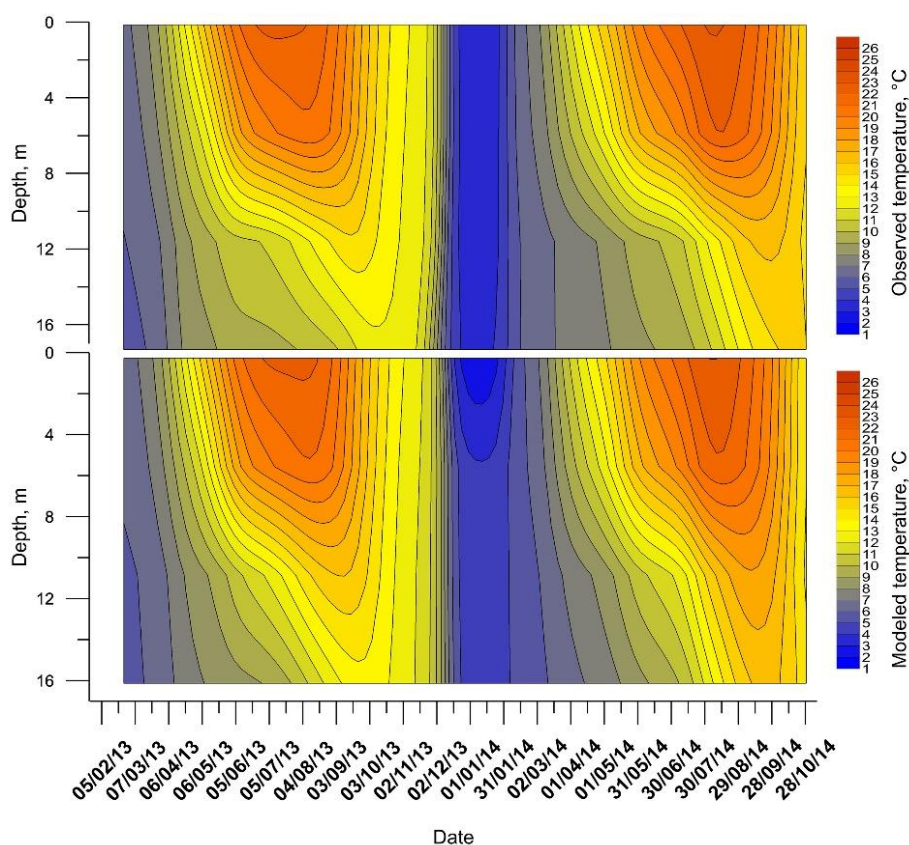
Figure 8. Temperature isopleths according to time (observation and model results)
