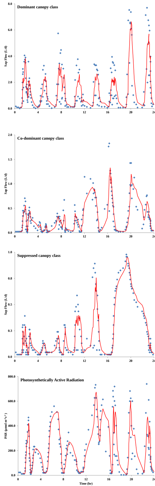
Figure 5. The daily curves of Sap flow ( \text{Lh}^{-1} ) and PAR for the three canopy classes of J. macrocarpa
