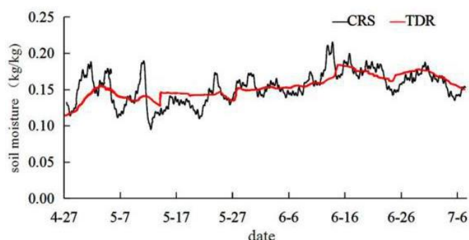
Figure 2. The comparison of CRS and TDR soil moisture in experiment period
