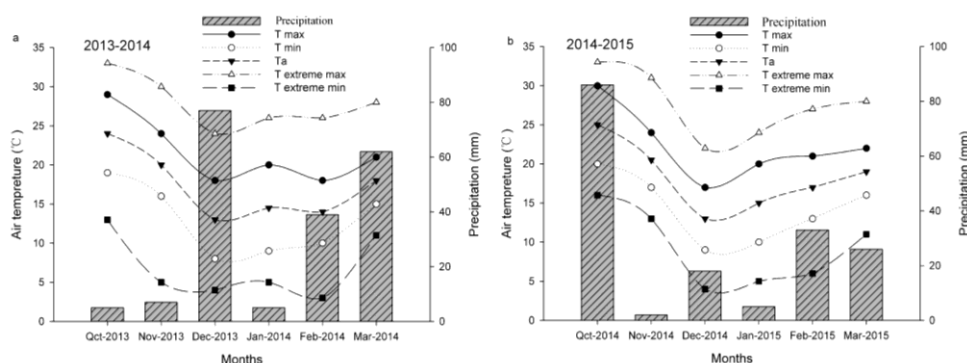
Figure 2. Average monthly air temperature and precipitation during the potato growing season in 2013~2014 and 2014~2015. T max: maximum average monthly air temperature; T min: minimum average monthly air temperature; Ta: average monthly air temperature. T extreme max: extreme maximum average monthly air temperature; T extreme min: extreme minimum average monthly air temperature
