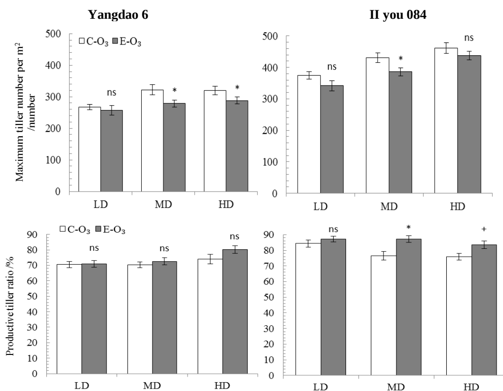
Figure 7. Effects of surface ozone concentration and plant density on maximum tiller number per square meter and productive tiller ratio of Yangdao 6 and II-you 084. ANOVA (M means maximum tiller number per square meter, P means productive tiller ratio): M: Cultivar ( P < 0.01 ); Density ( P < 0.01 ); Ozone ( P < 0.01 ); O 3 × C ( p > 0.1 ); O 3 × D ( p > 0.1 ); C × D ( p > 0.1 ); O 3 × C × D ( p > 0.1 ). P: Cultivar ( P < 0.01 ); Density ( p > 0.1 ); Ozone ( P < 0.05 ); O 3 × C ( p > 0.1 ); O 3 × D ( p > 0.1 ); C × D ( p > 0.1 ); O 3 × C × D ( p > 0.1 ).
