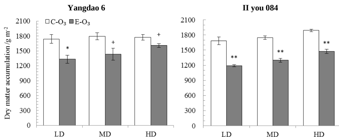
Figure 4. Effects of surface ozone concentration and plant density on biomass yield of Yangdao 6 and II you 084. ANOVA: Cultivar ( P < 0.05 ); Density ( P < 0.01 ); Ozone ( P < 0.01 ); O_3 \times Cultivar ( P < 0.05 ); O_3 \times Density ( P < 0.1 ); Cultivar \times Density ( p > 0.1 ); O_3 \times Cultivar \times Density ( p > 0.1 )
