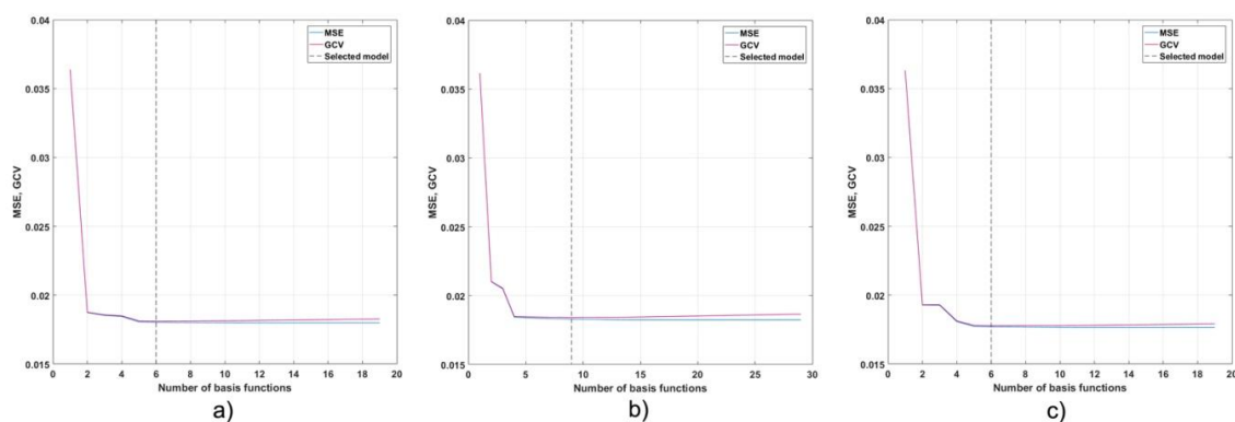
Figure 8. MSE vs. GCV values for the MARS models of a) R1-R2, b) R1-R3, and c) R2-R3
