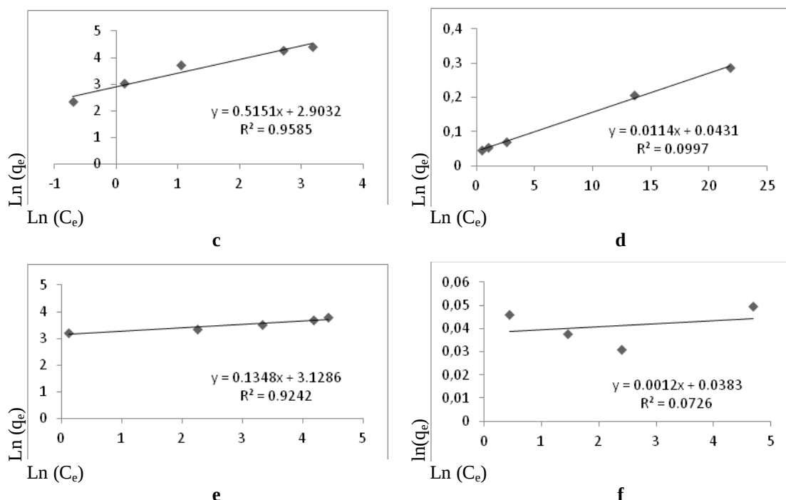
Figure 6. Adsorption isotherm of graphene oxide: a) Freundlich Cr(III), b) Langmuir Cr(III), c) Freundlich \text{Cd}^{2+} , d) Langmuir \text{Cd}^{2+} , e) Freundlich \text{Pb}^{2+} ion, and f) Langmuir \text{Pb}^{2+}
