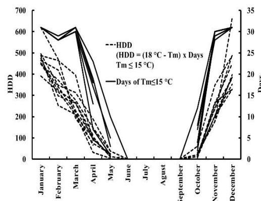
Figure 2. Change of HDD and T < 15\text{ }^{\circ}\text{C} days between 2008-2017 by months
