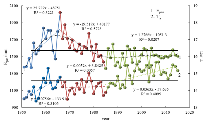
Figure 6. Variations of the average annual E_{\text{pan}} and T_a in the HRB (the dotted curve is the six-year moving average of E_{\text{pan}} , the dotted lines represent the linear trends fitted to the corresponding periods)
