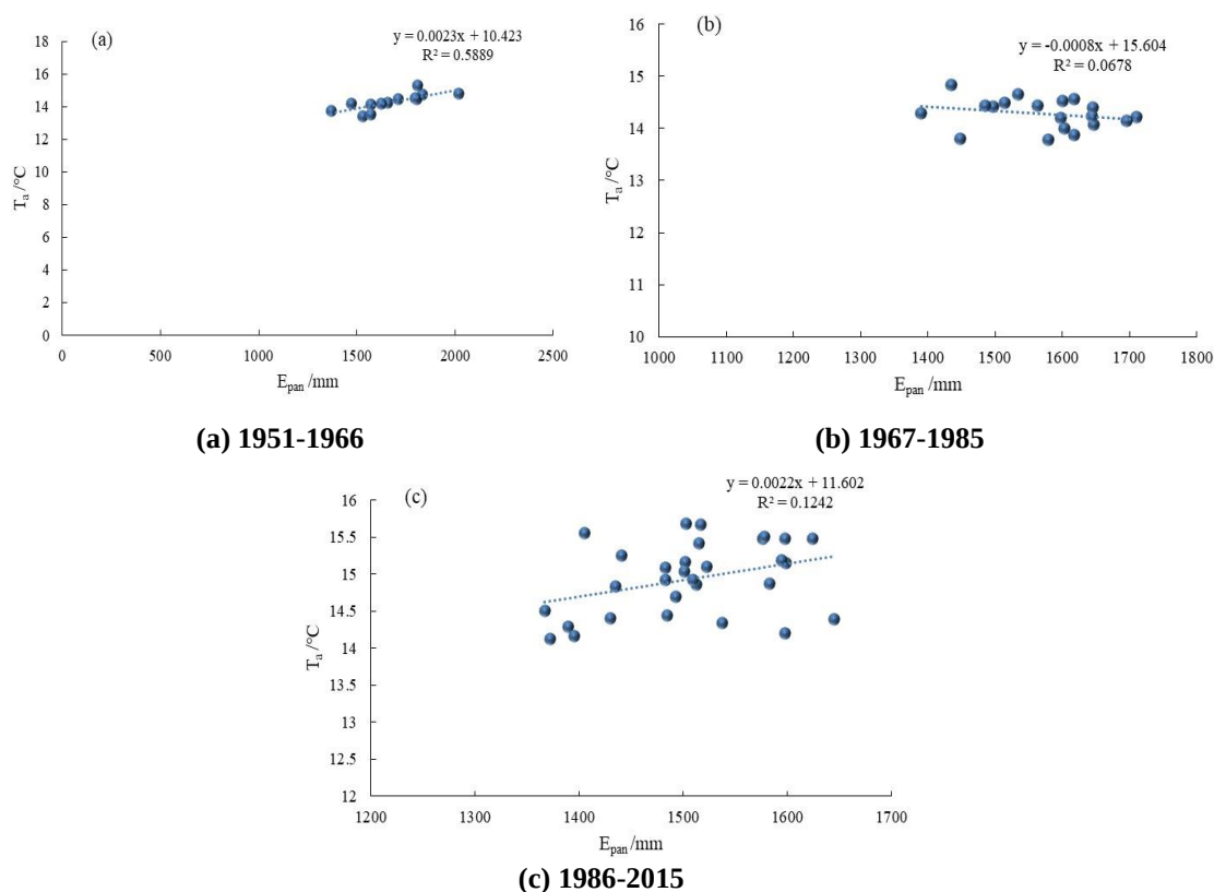
Figure 7. Scatter plots between E_{\text{pan}} and T_a of the HRB during different periods
