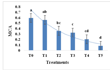
Figure 5. Variation among root-shoot ratio (a), biomass production (kg) (b), and moisture content availability (kg) (c) under different soil compaction levels (*significant, **highly significant, NS non-significant)
