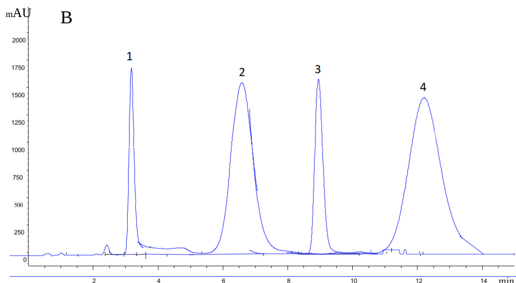
Figure 6. Typical chromatograms: (A) water sample spiked with \text{Cr}^{2+} , \text{Ni}^+ , \text{Co}^{2+} and \text{Hg}^+ without dispersive liquid-liquid microextraction-magnetic solid phase extraction and (B) after dispersive liquid-liquid microextraction-magnetic solid phase extraction. 1, \text{Cr}^{2+} ; 2, \text{Ni}^+ ; 3, \text{Co}^{2+} ; 4, \text{Hg}^+
