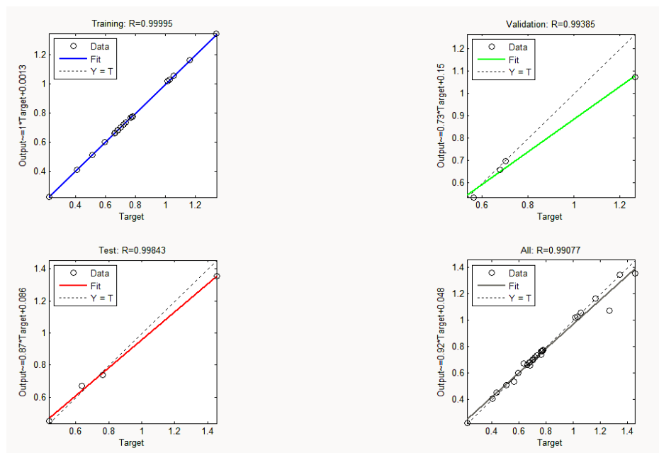
Figure 3. Evaluation models for WQI for recurrent neural network
