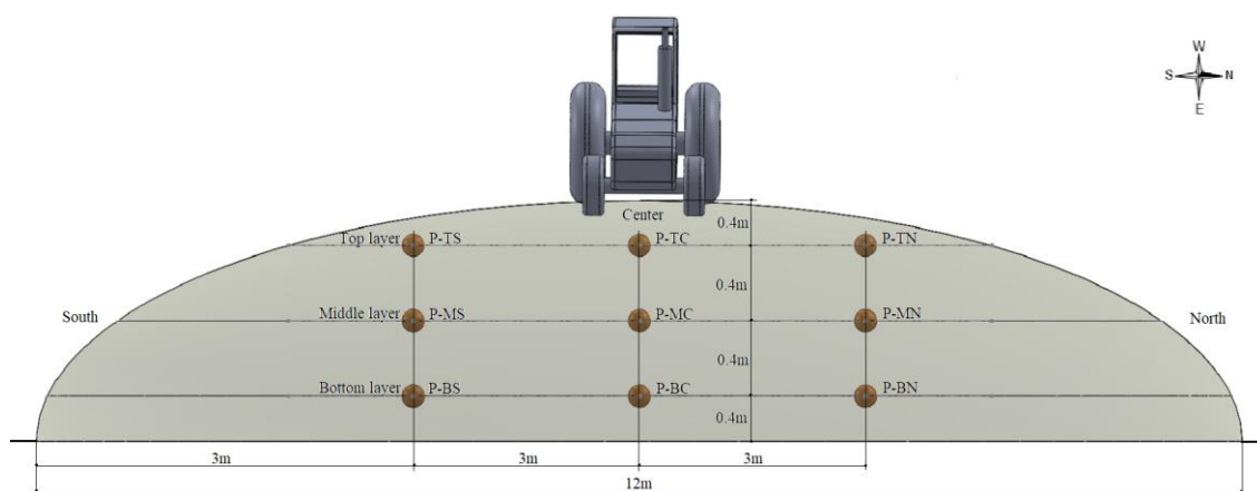
Figure 1. Pressure measurement points in the pile silos
