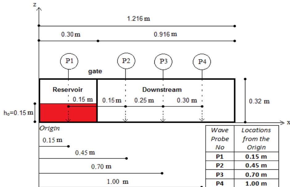
Figure 3. Channel measurement points
