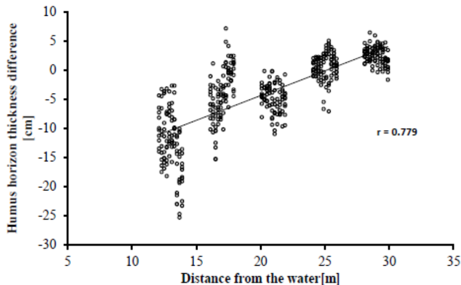
Figure 14. Dependence of the humus horizon thickness difference on the distance from the water body
